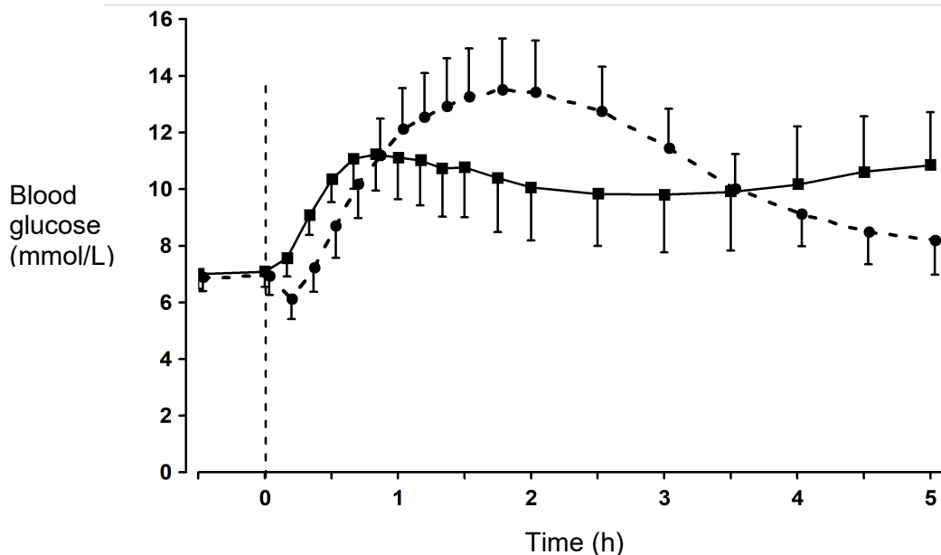
Figure 1: Blood glucose concentrations* (mean \pm 2SEM) following a single pre-meal dose (0.15 U/kg) of NovoRapid injected immediately before a meal (solid curve) or soluble human insulin administered 30 minutes before a meal (dashed curve) in patients with type 1 diabetes mellitus.
